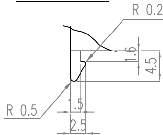
"E" DETAIL 2/1
