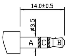
MATING PLUG
