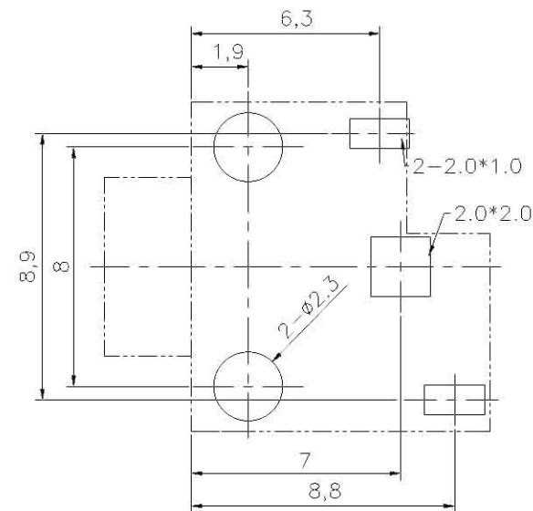
P.C.B. HOLE LAYOUT (BOTTOM VIEW)
