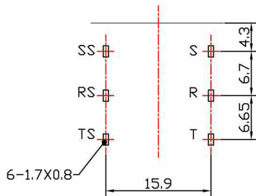
PCB MOUNTING HOLES (VIEWED FROM COPPER SIDE)
