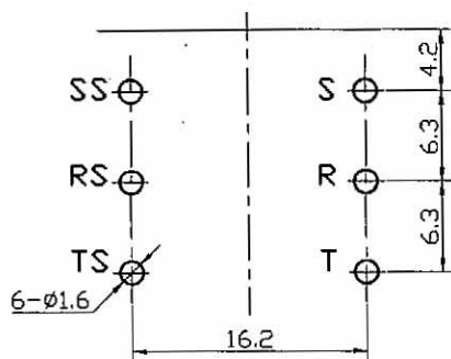
PCB MOUNTING HOLES (VIEWED FROM COPPER SIDE)
