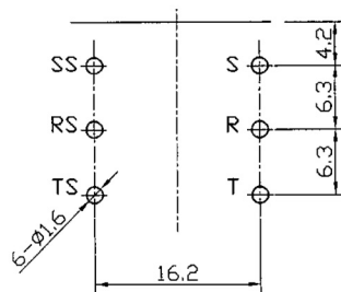
PCB MOUNTING HOLES (VIEWED FROM COPPER SIDE)
