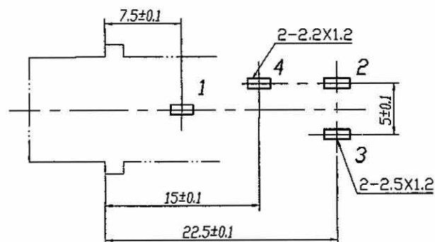
PCB MOUNTING HOLES (BOTTOM VIEW) Tolerance: ±0.1
