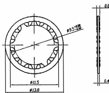
WASHER
