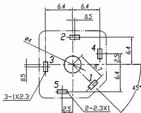
PCB MOUNTING HOLES (VIEWED FROM COPPER SIDE)
