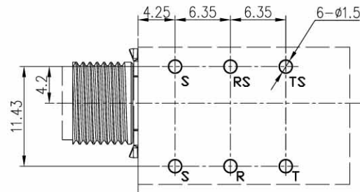
PCB MOUNTING HOLES (TOP VIEW) Tolerance: ± 0.05
