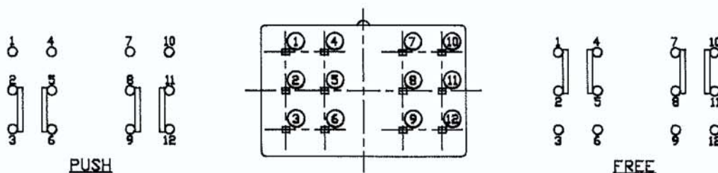
SCHEMATIC
