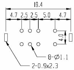
PCB LAYOUT
