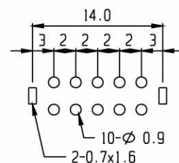
PCB LAYOUT
