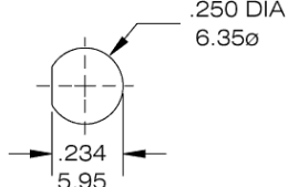
flatted D
