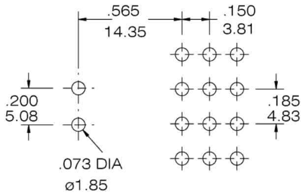
PCB Footprint
