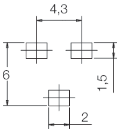
PCB Layout
