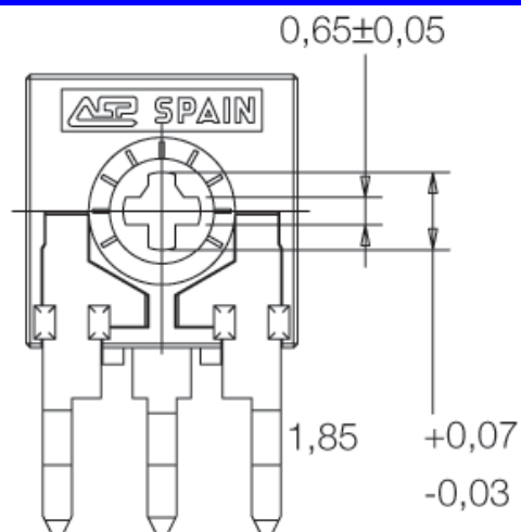
Standard Rotor ('X')
